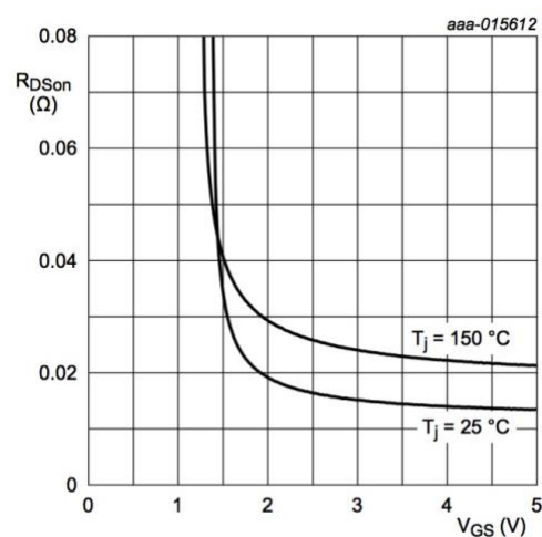
Fig.2 On-Resistance vs. Gate-Source
